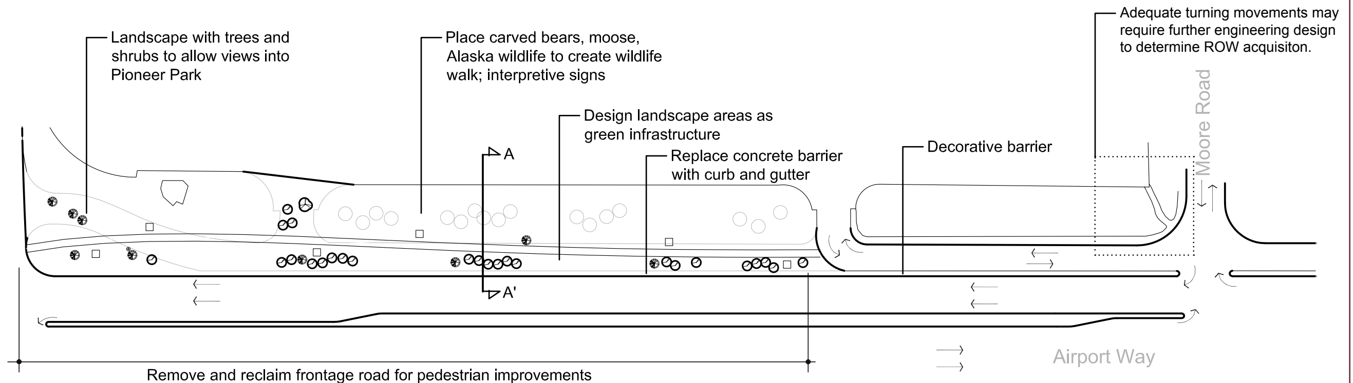
Site Plan
